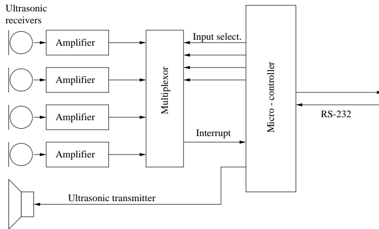
Figure 2: Schematic diagram
