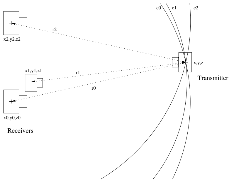
Figure 1: Working arrangement
